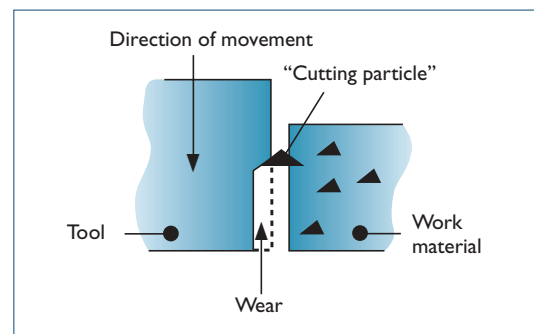
Figure 2. Schematic representation of abrasive wear.
